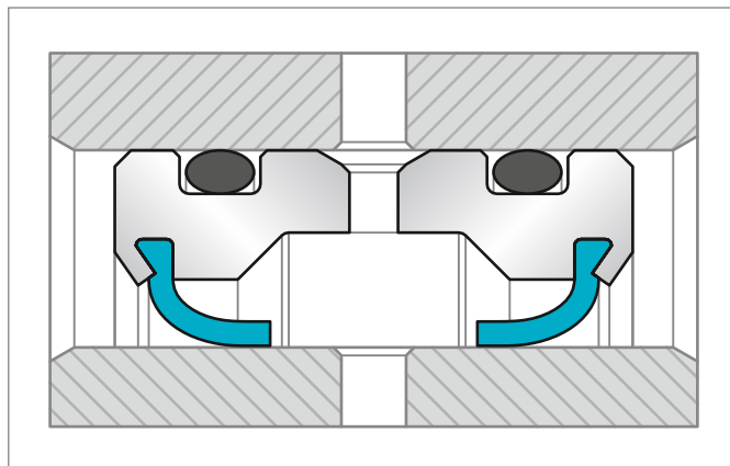
Figure 5: Fluid Transfer. Injection ports enable the transfer of fluid between the housing and the shaft.
