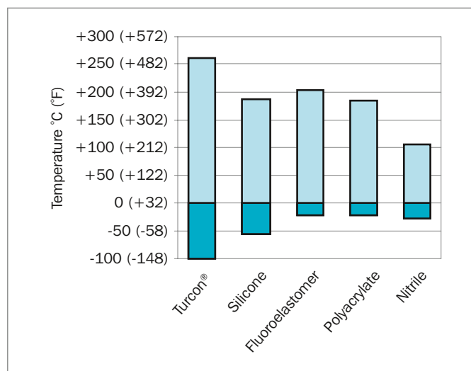
Figure 9: Maximum and minimum temperatures for different materials
