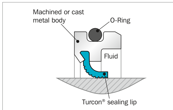
Figure 3: O-Ring Design. For low interference fits in the housing. Housing surface finish > 0.8 \mu\text{m Ra} or particularly searching media control.
