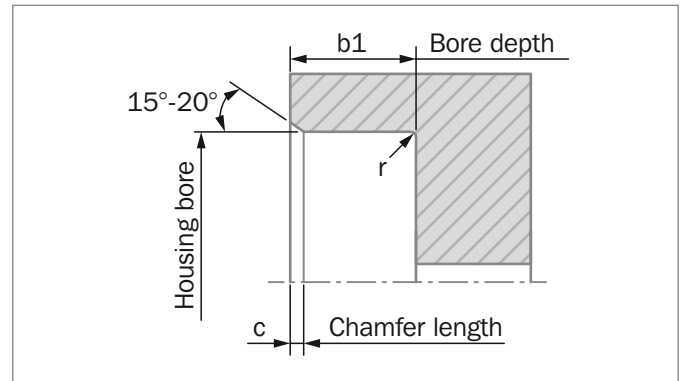
Figure 13: Housing design schematic
