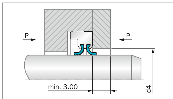
Figure 21: Installation type for fluid separation (Type D) at pressures up to 0.5 MPa (73 psi).
