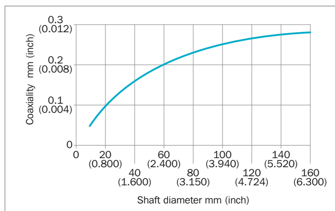
Figure 12: Coaxial tolerance capability
