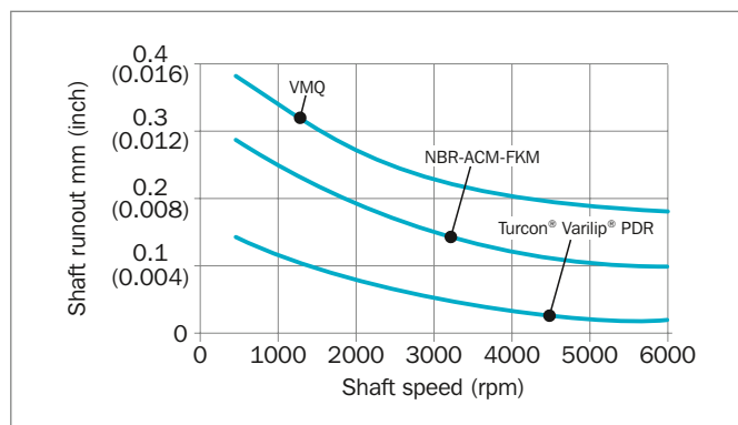
Figure 11: Dynamic eccentricity capability
