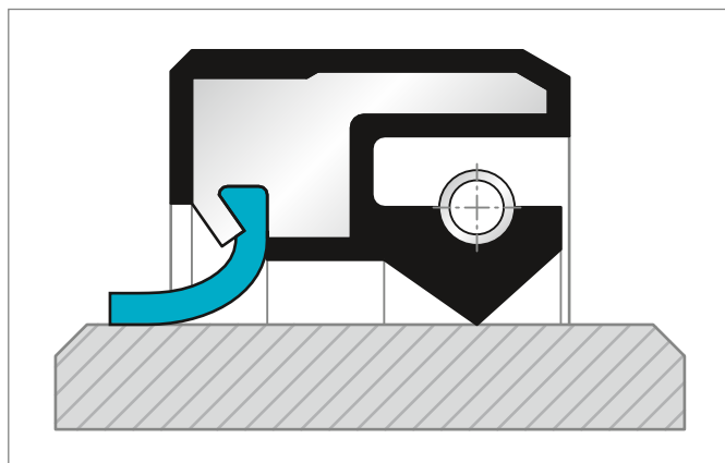
Figure 7: Elastomer/Turcon® Hybrid. This combination utilizes the best attributes of both a Radial Oil Seal and the Turcon® Varilip® PDR.
