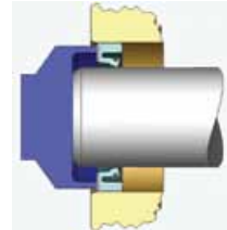
Installation Method C Thru Bore:
