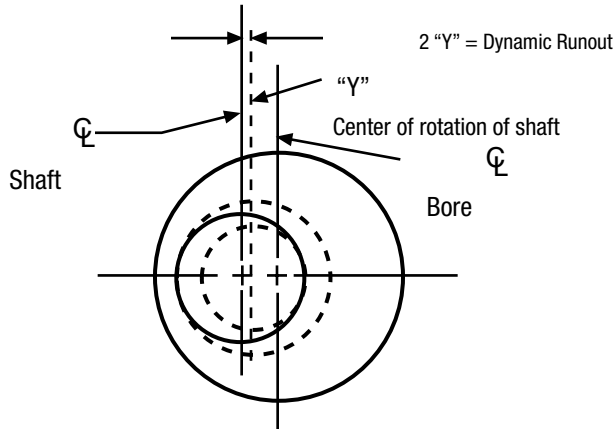
Figure 6 — Dynamic Runout
